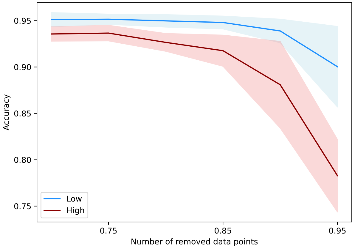
DataAttrOpt(5000, 0.02, 15, max+s, alpha=0.5) - bbc-embeddings
